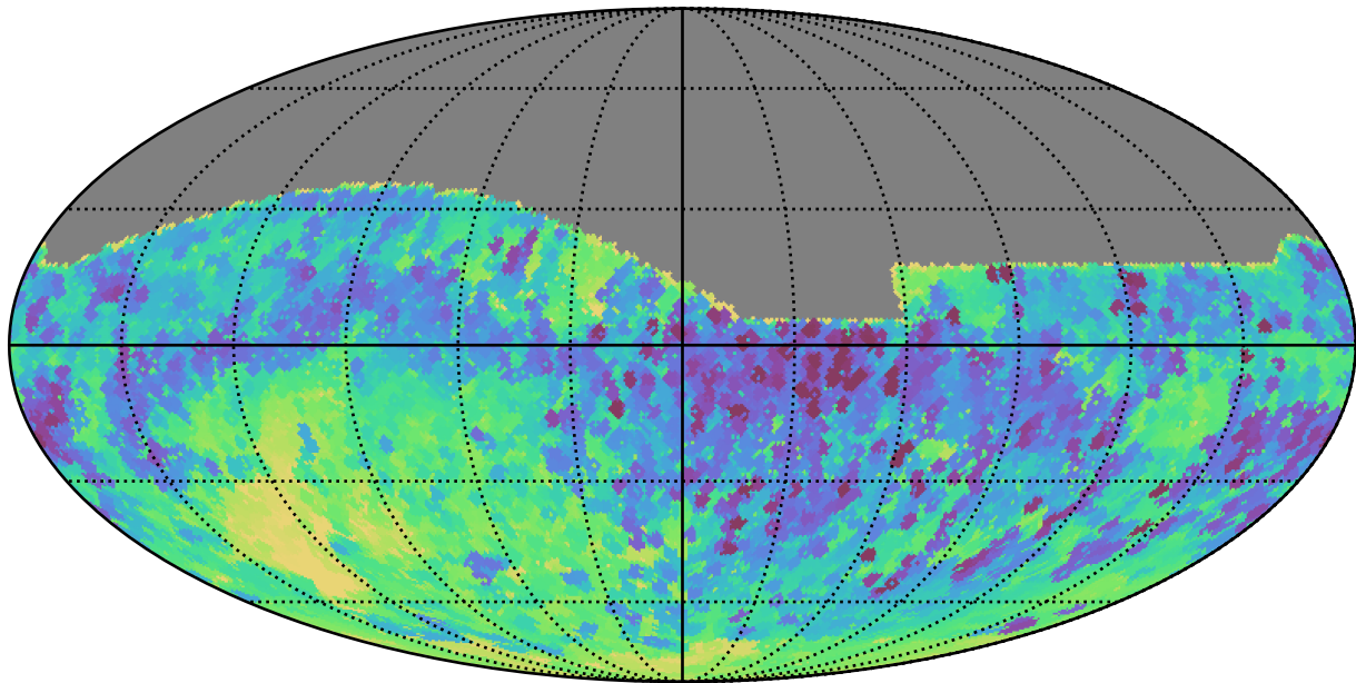
baseline_v3.0_10yrs All sky z band: Min skyBrightness
