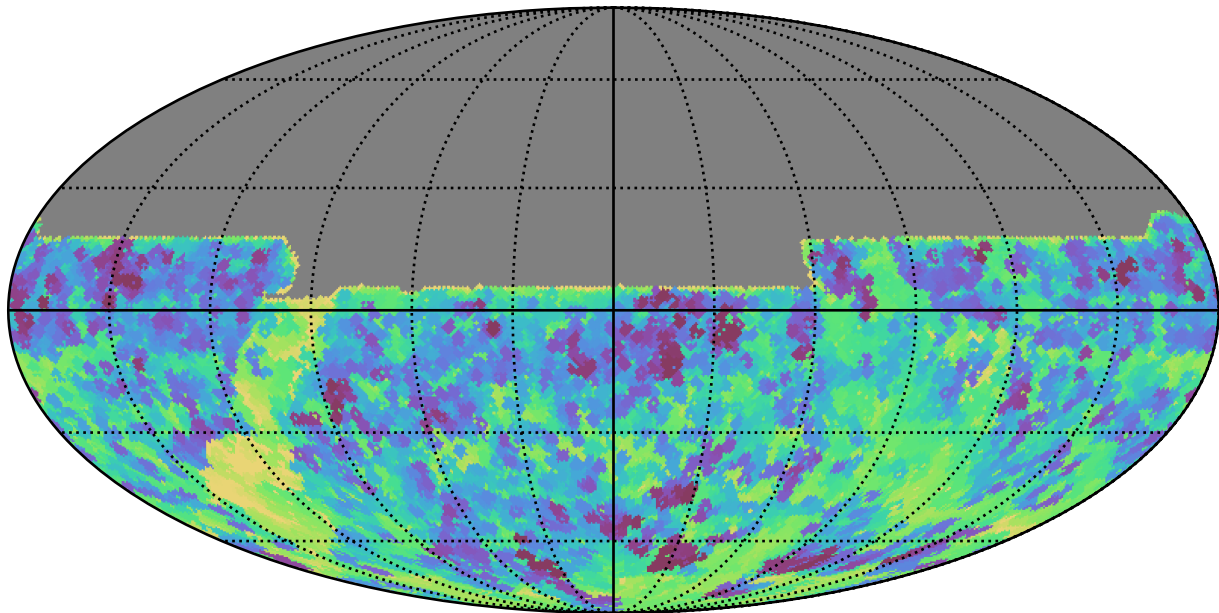
baseline_v3.0_10yrs All sky y band: Min skyBrightness
