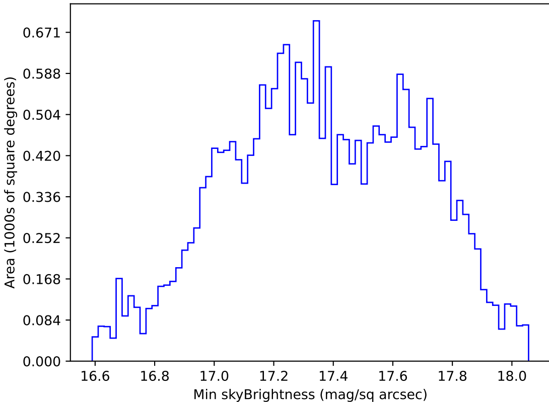
baseline_v3.0_10yrs All sky y band: Min skyBrightness
