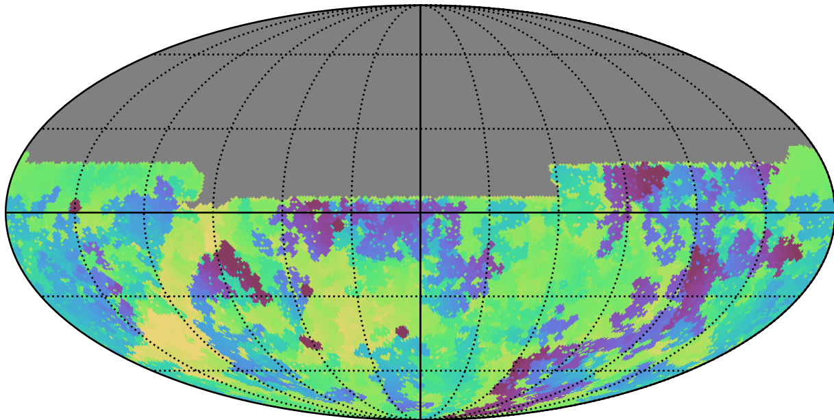
baseline_v3.0_10yrs All sky u band: Min skyBrightness
