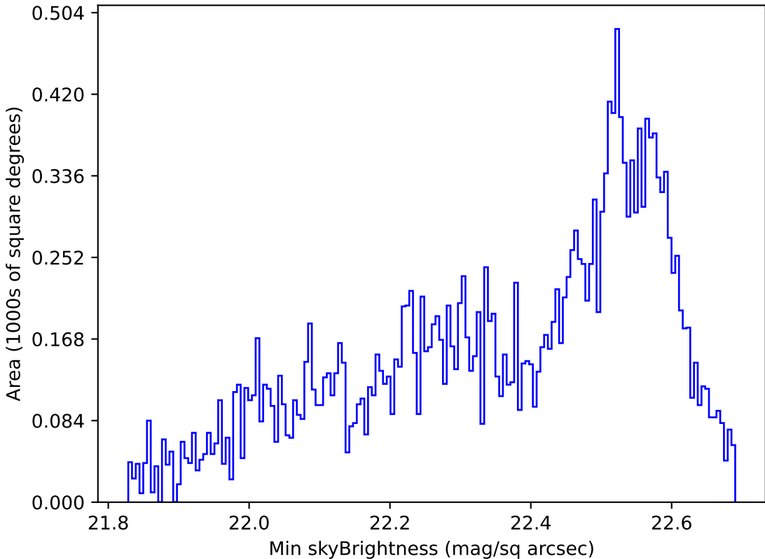
baseline_v3.0_10yrs All sky u band: Min skyBrightness
