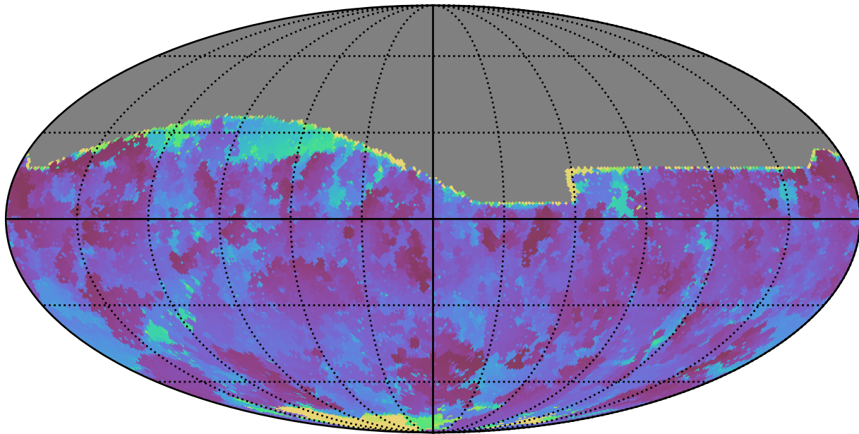
baseline_v3.0_10yrs All sky r band: Min skyBrightness
