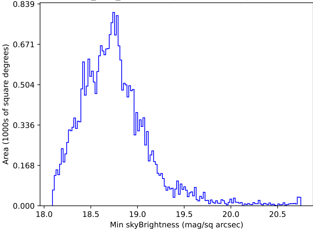
baseline_v3.0_10yrs All sky r band: Min skyBrightness
