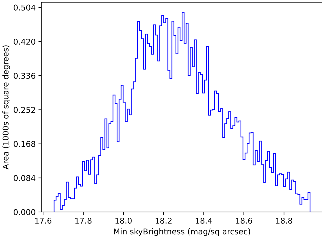
baseline_v3.0_10yrs All sky i band: Min skyBrightness
