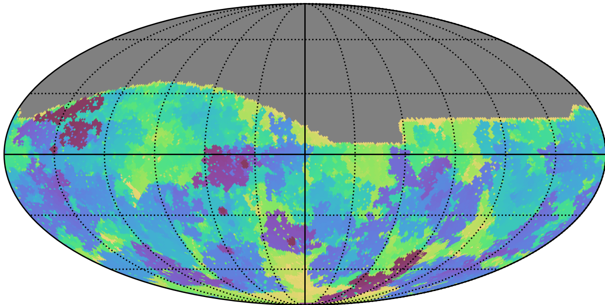
baseline_v3.0_10yrs All sky g band: Min skyBrightness
