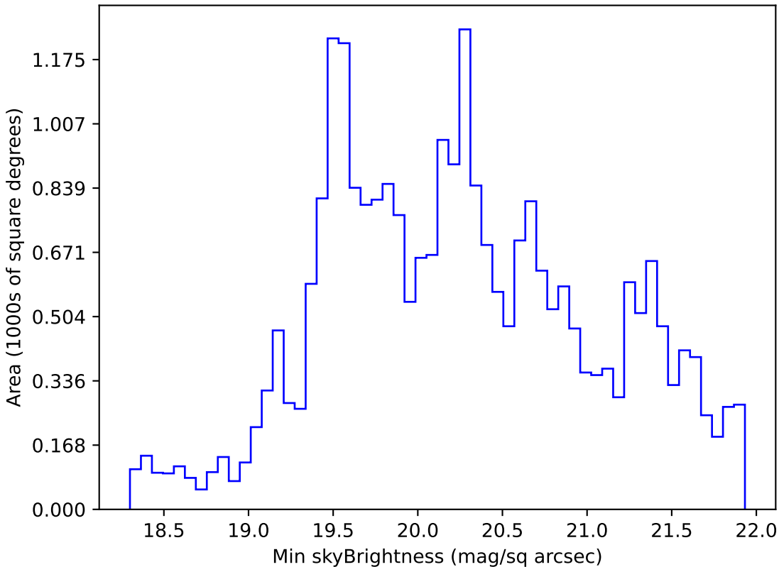
baseline_v3.0_10yrs All sky g band: Min skyBrightness
