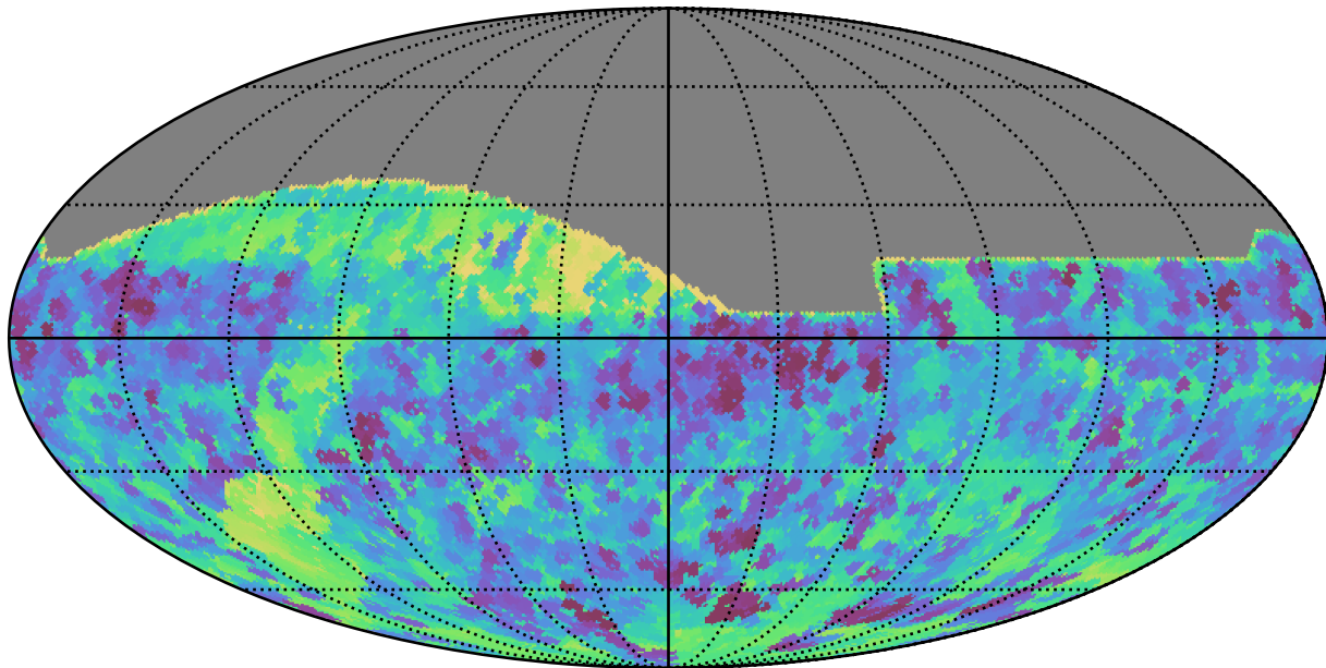
baseline_v3.0_10yrs All sky all bands: Min skyBrightness
