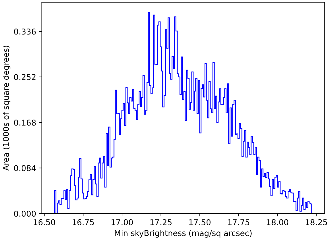
baseline_v3.0_10yrs All sky all bands: Min skyBrightness
