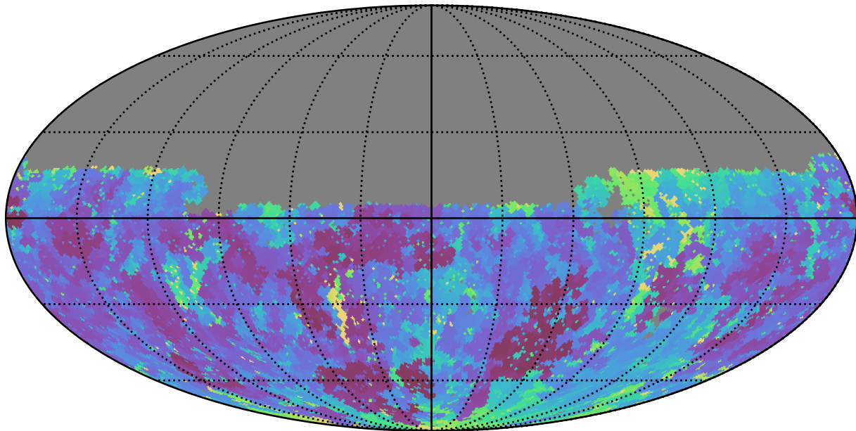
baseline_v3.0_10yrs Yr 1 u band: Min seeingGeom
