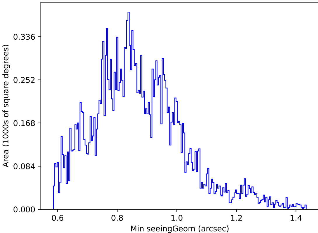
baseline_v3.0_10yrs Yr 1 u band: Min seeingGeom
