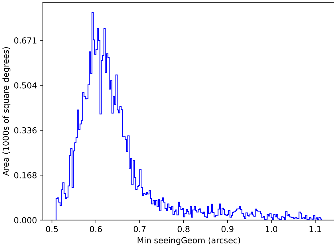
baseline_v3.0_10yrs Yr 1 r band: Min seeingGeom
