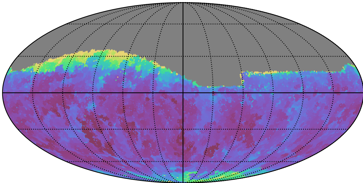
baseline_v3.0_10yrs Yr 1 i band: Min seeingGeom
