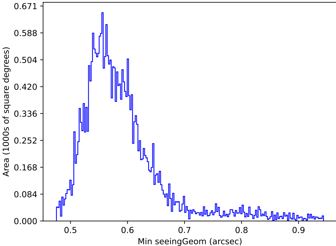
baseline_v3.0_10yrs Yr 1 all bands: Min seeingGeom
