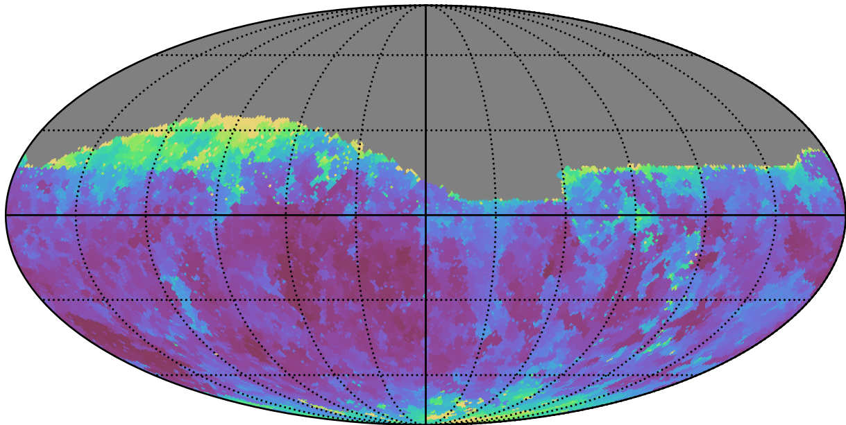
baseline_v3.0_10yrs Yr 1 z band: Min seeingEff
