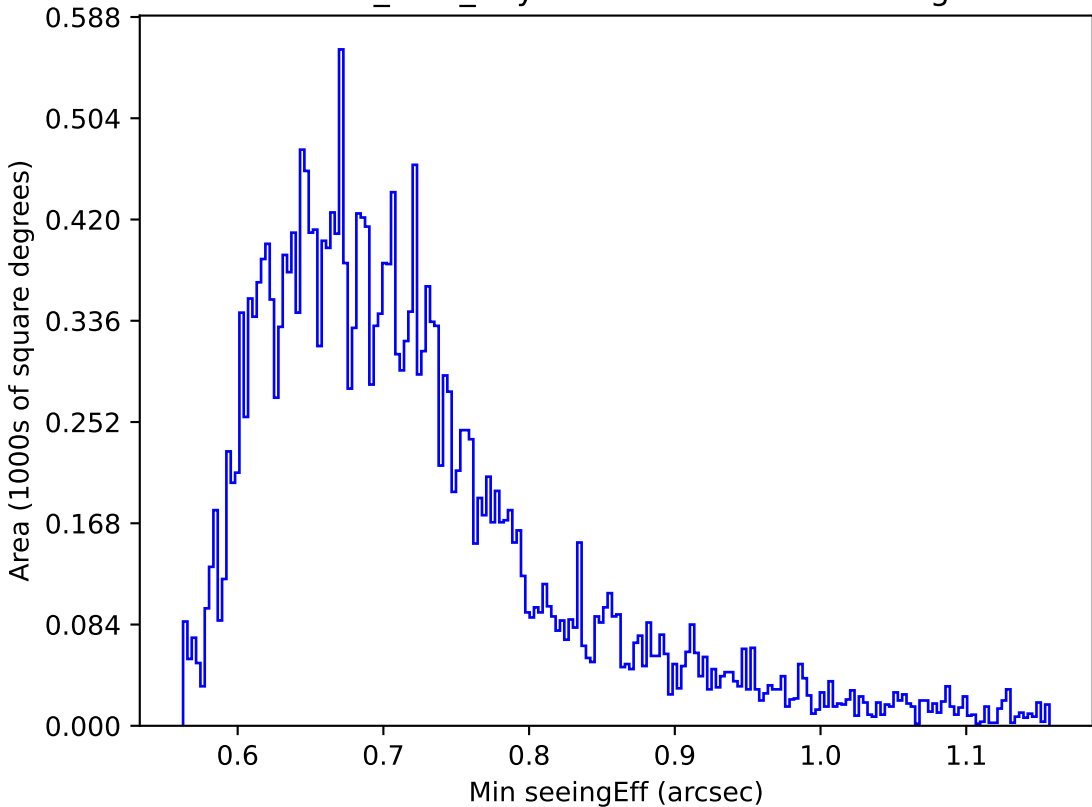
baseline_v3.0_10yrs Yr 1 z band: Min seeingEff
