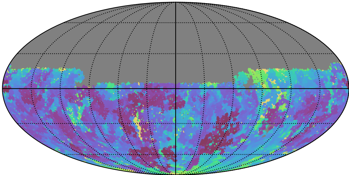
baseline_v3.0_10yrs Yr 1 u band: Min seeingEff
