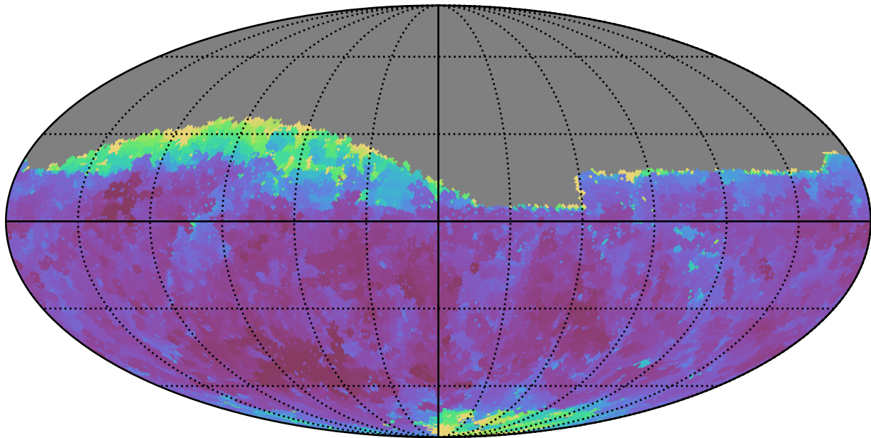
baseline_v3.0_10yrs Yr 1 r band: Min seeingEff
