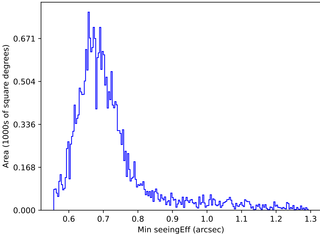
baseline_v3.0_10yrs Yr 1 r band: Min seeingEff
