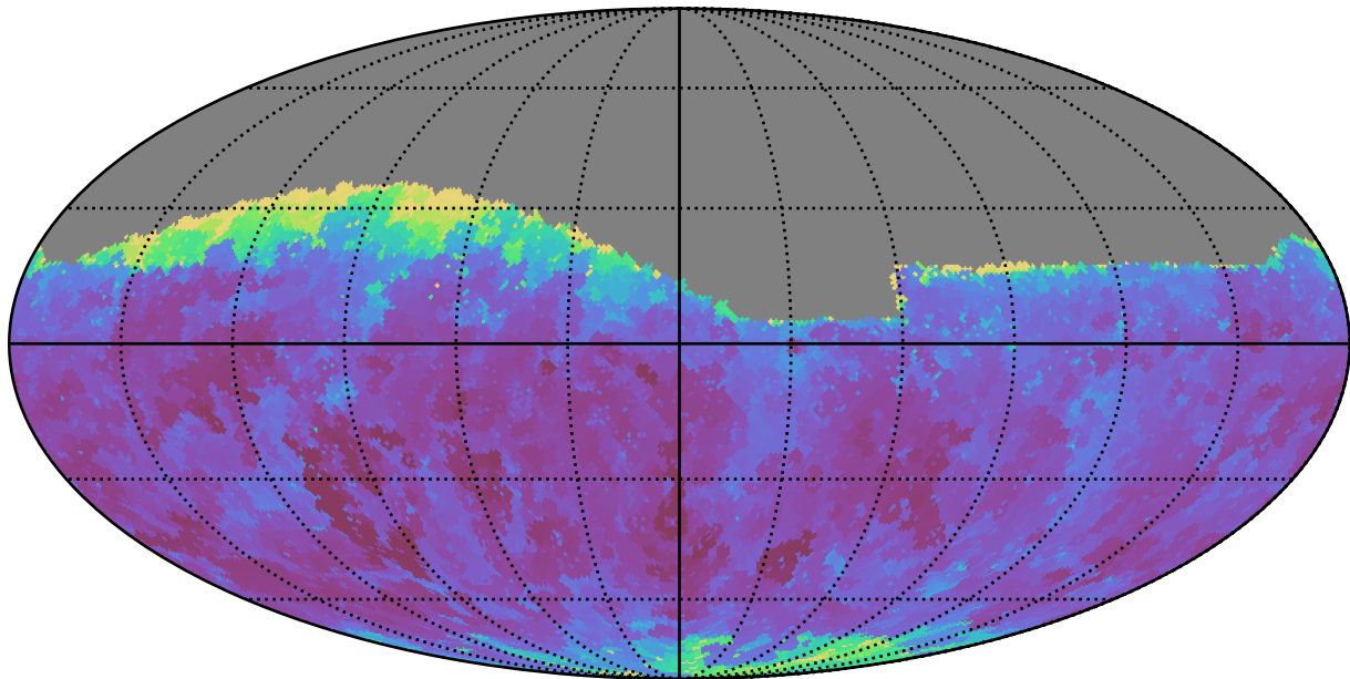
baseline_v3.0_10yrs Yr 1 i band: Min seeingEff
