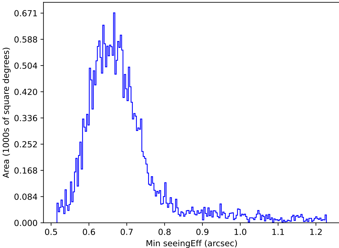
baseline_v3.0_10yrs Yr 1 i band: Min seeingEff
