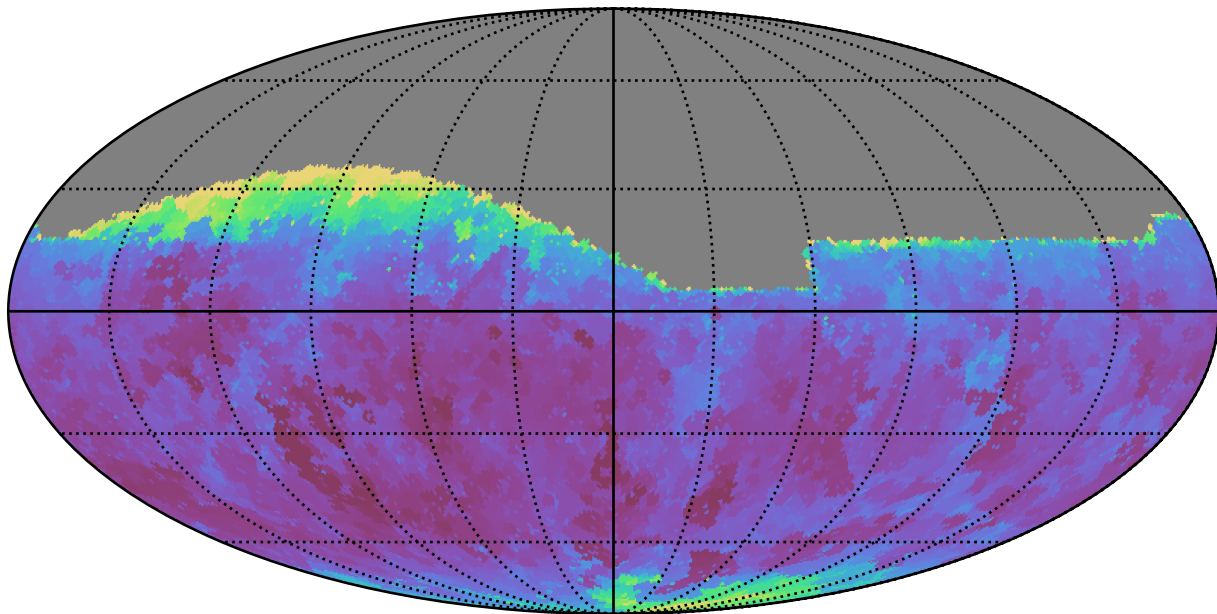
baseline_v3.0_10yrs Yr 1 all bands: Min seeingEff
