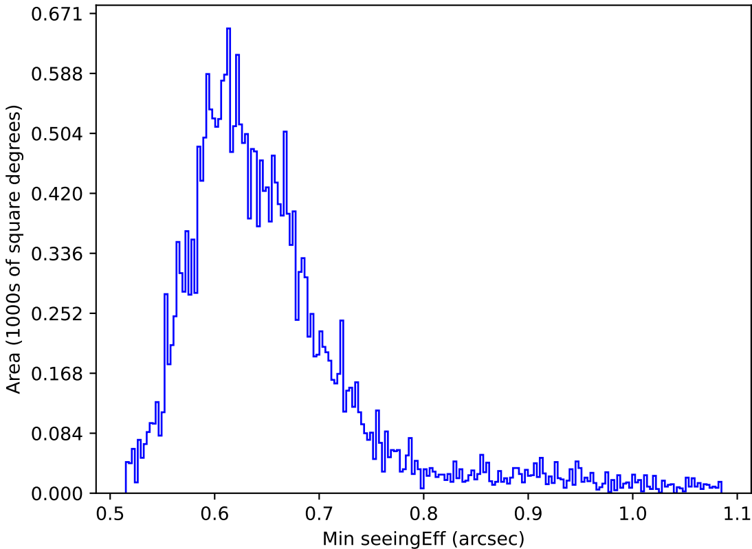
baseline_v3.0_10yrs Yr 1 all bands: Min seeingEff
