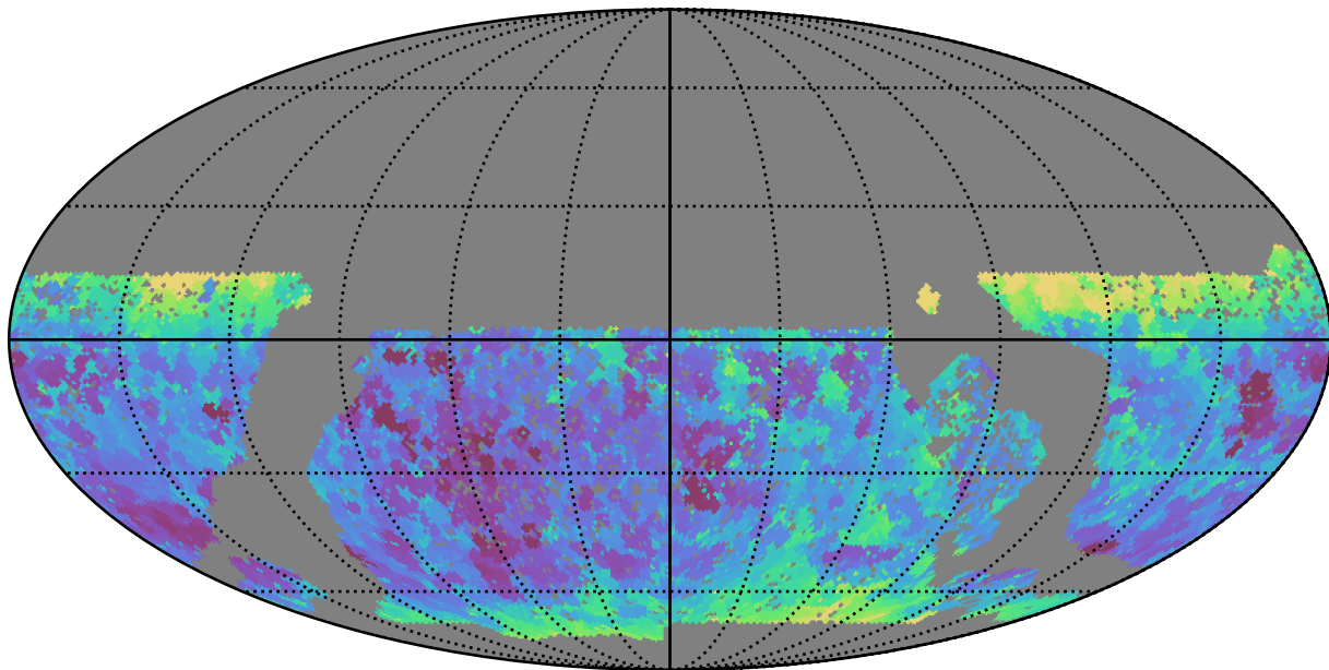
baseline_v3.0_10yrs WFD z band: Min seeingEff
