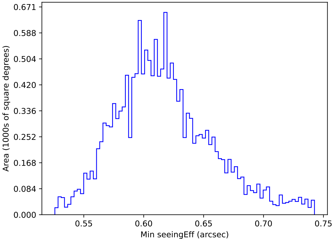
baseline_v3.0_10yrs WFD z band: Min seeingEff
