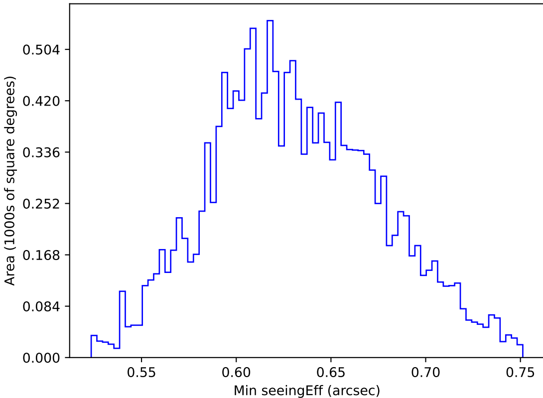
baseline_v3.0_10yrs WFD y band: Min seeingEff
