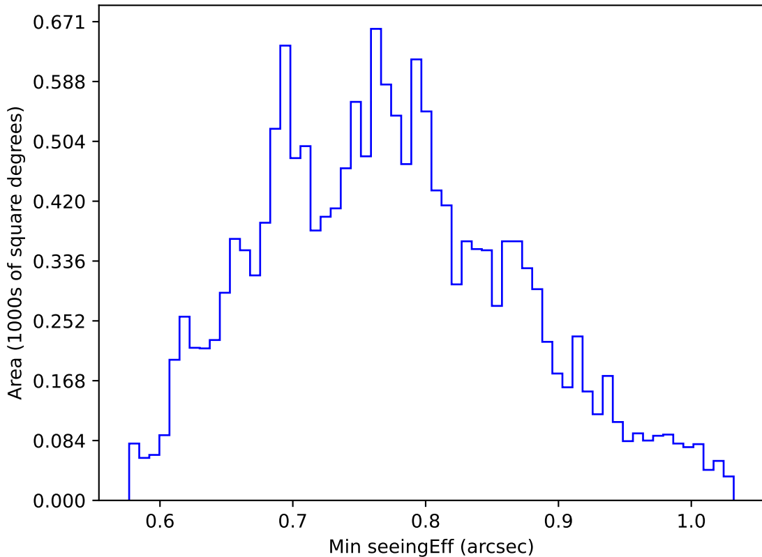
baseline_v3.0_10yrs WFD u band: Min seeingEff
