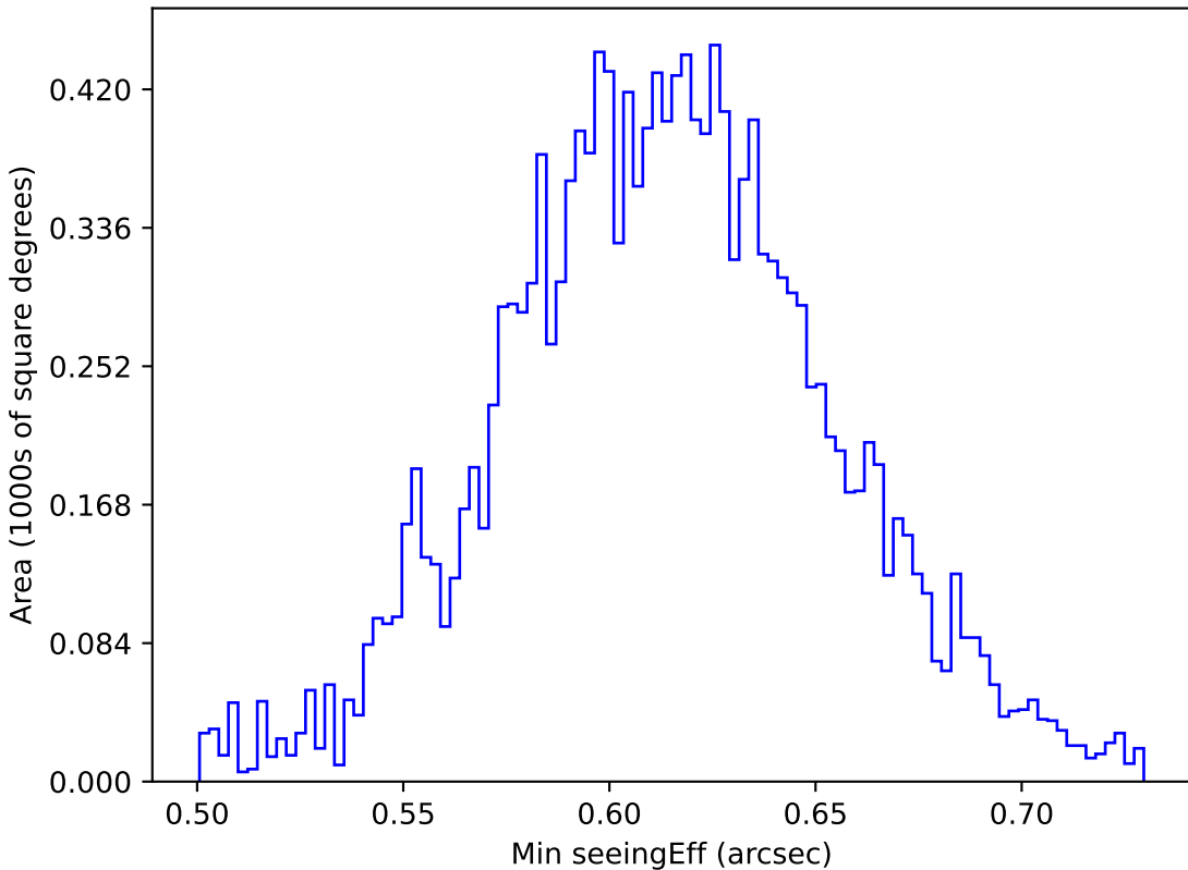
baseline_v3.0_10yrs WFD r band: Min seeingEff
