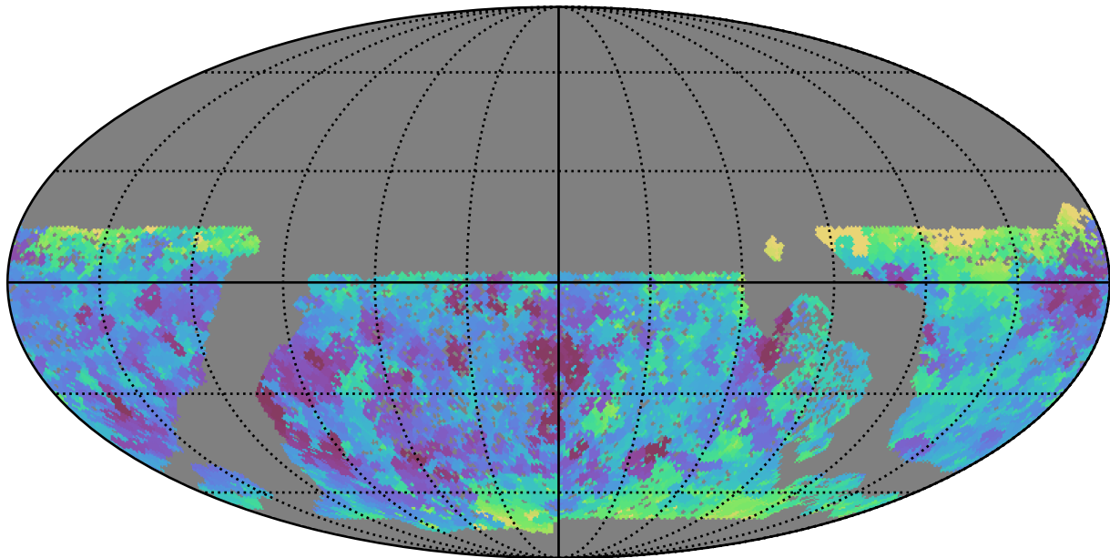
baseline_v3.0_10yrs WFD i band: Min seeingEff
