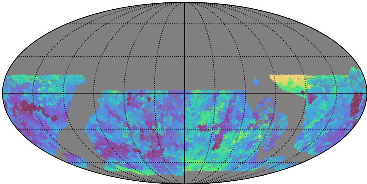
baseline_v3.0_10yrs WFD g band: Min seeingEff
