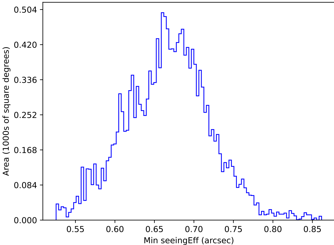
baseline_v3.0_10yrs WFD g band: Min seeingEff
