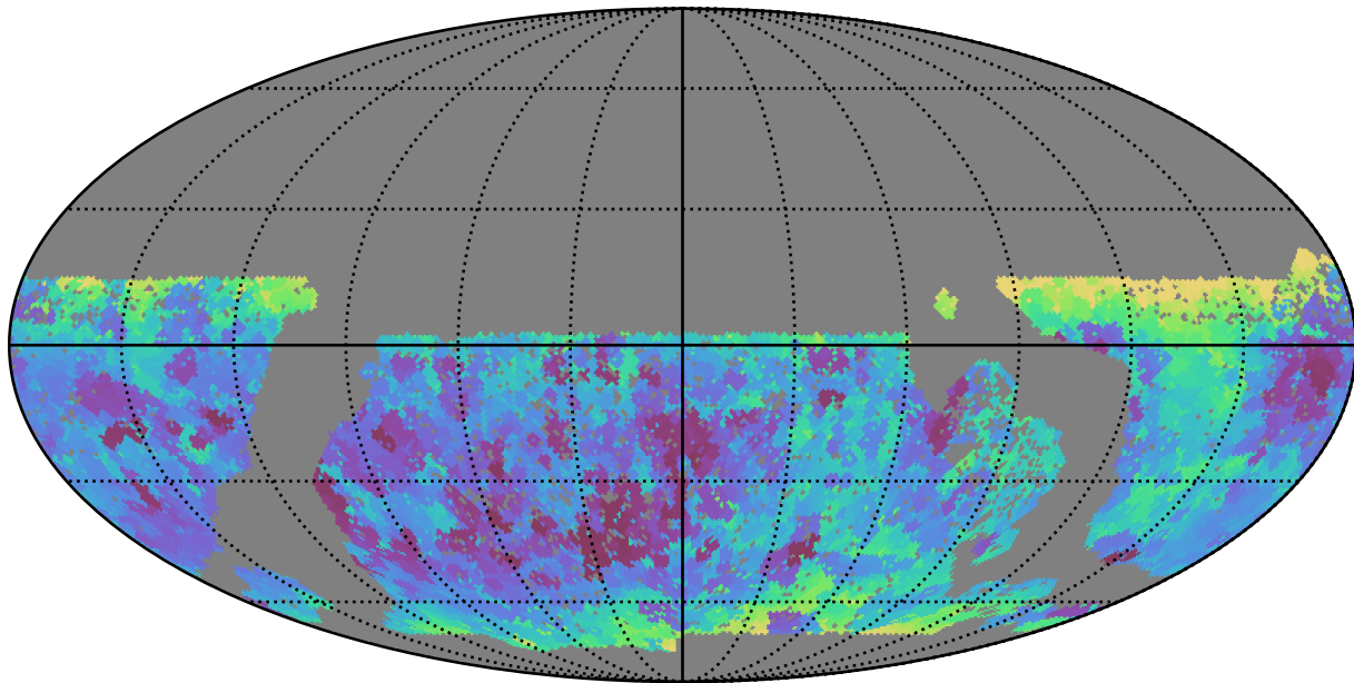
baseline_v3.0_10yrs WFD all bands: Min seeingEff
