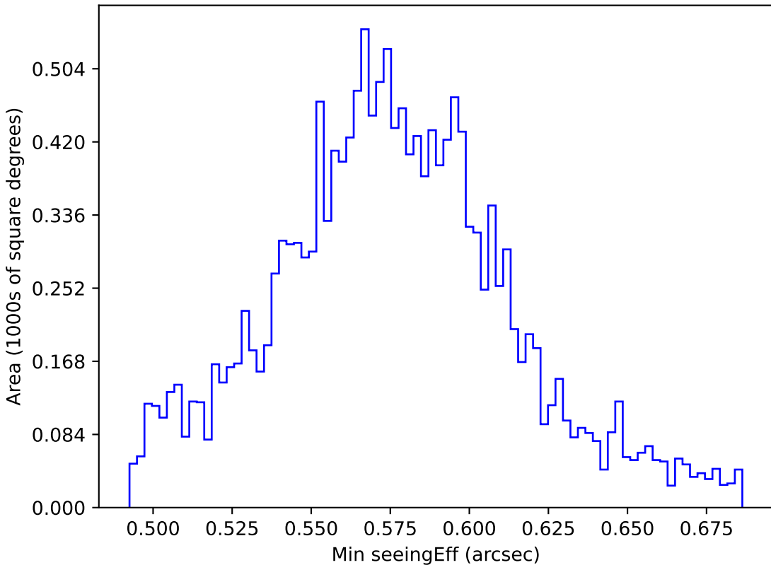
baseline_v3.0_10yrs WFD all bands: Min seeingEff
