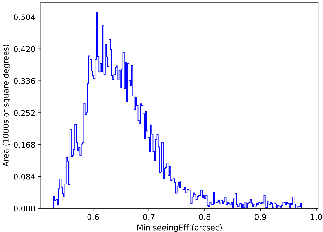
baseline_v3.0_10yrs All sky y band: Min seeingEff
