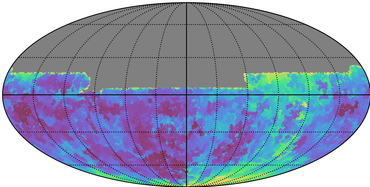
baseline_v3.0_10yrs All sky u band: Min seeingEff
