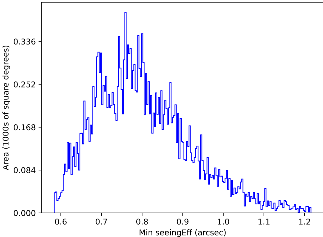
baseline_v3.0_10yrs All sky u band: Min seeingEff
