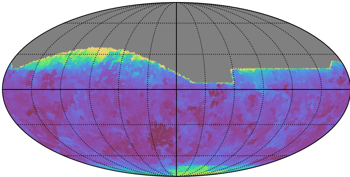
baseline_v3.0_10yrs All sky r band: Min seeingEff
