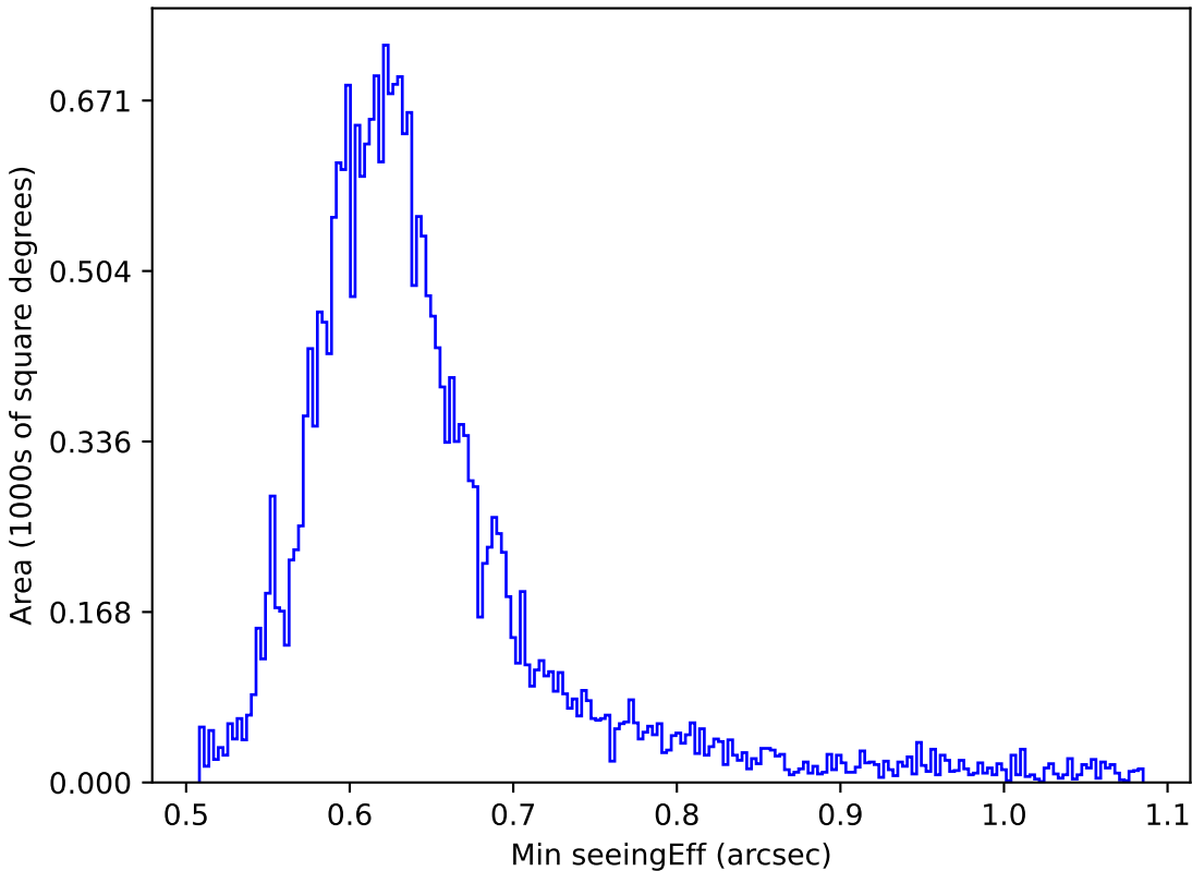
baseline_v3.0_10yrs All sky r band: Min seeingEff
