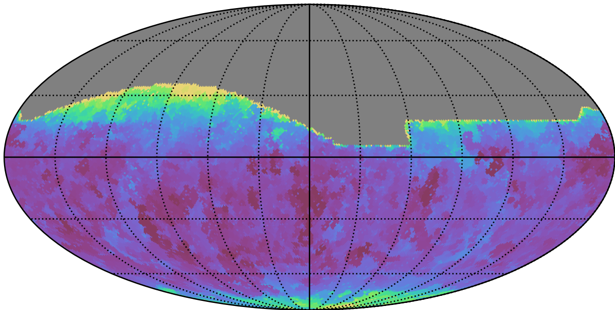
baseline_v3.0_10yrs All sky i band: Min seeingEff
