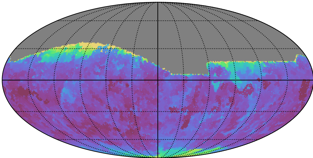
baseline_v3.0_10yrs All sky g band: Min seeingEff
