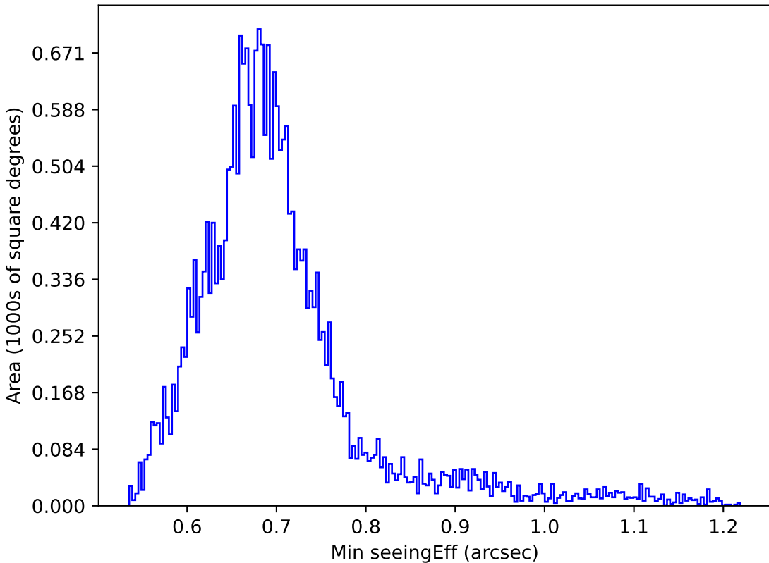
baseline_v3.0_10yrs All sky g band: Min seeingEff
