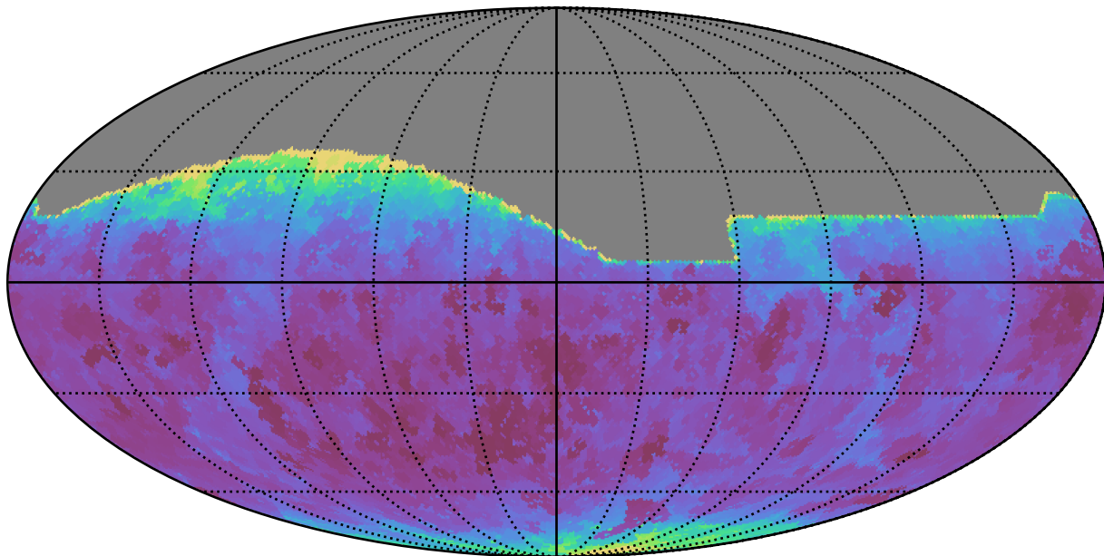
baseline_v3.0_10yrs All sky all bands: Min seeingEff
