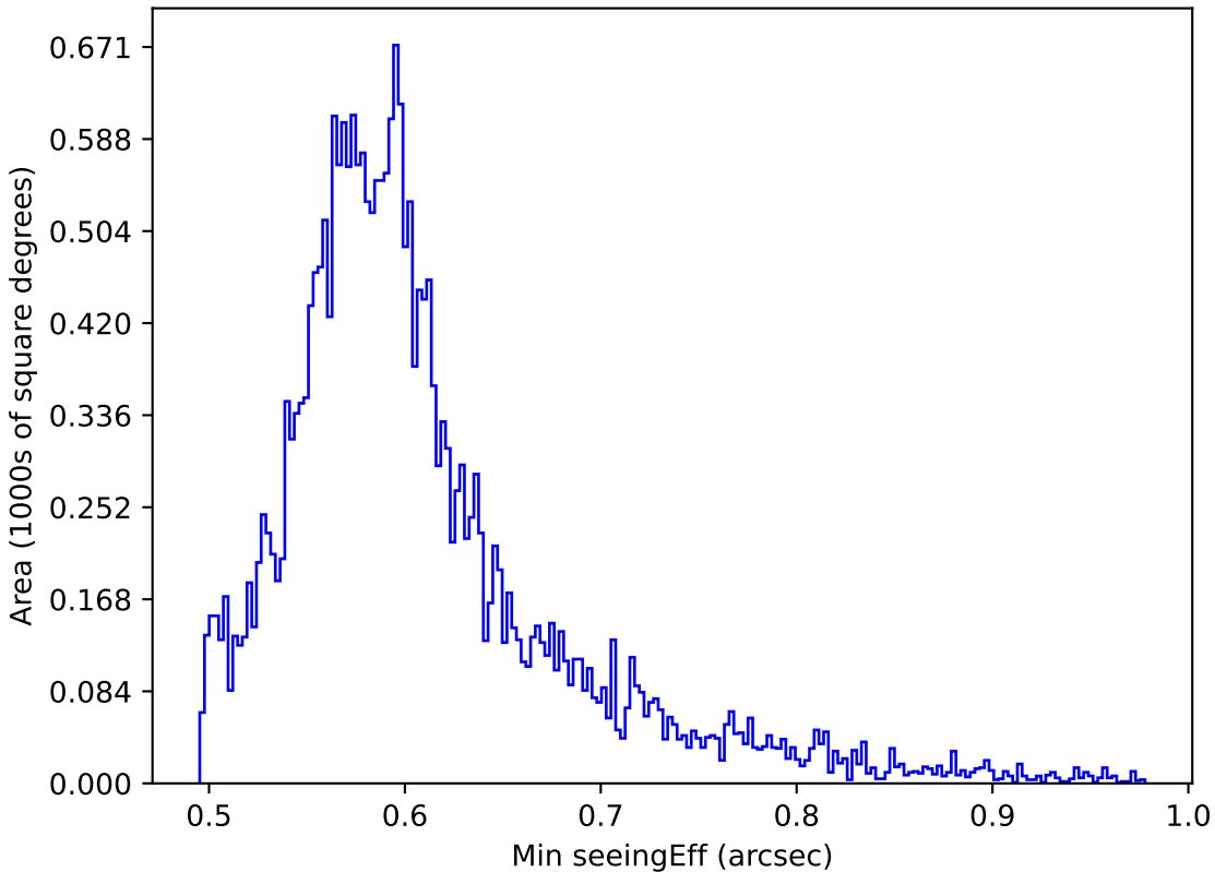
baseline_v3.0_10yrs All sky all bands: Min seeingEff
