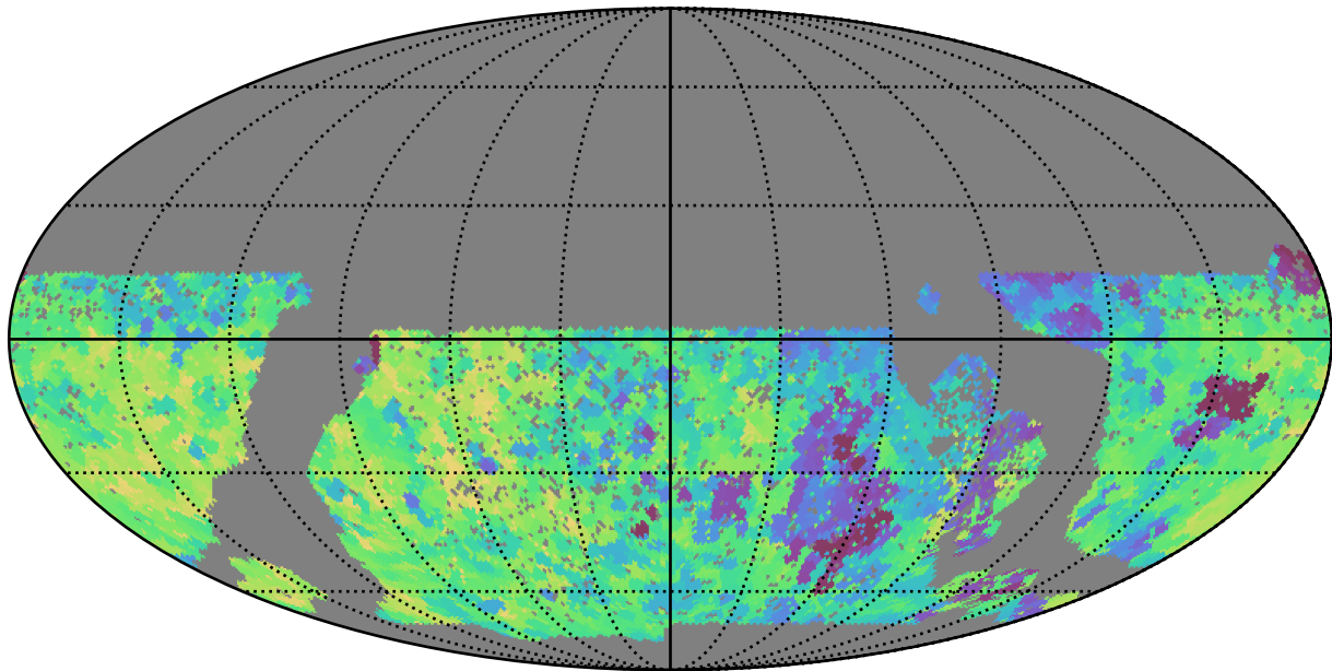
baseline_v3.0_10yrs WFD z band: Min saturation_mag
