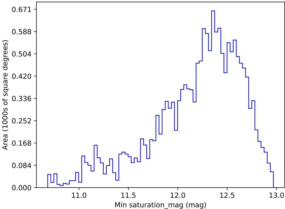
baseline_v3.0_10yrs WFD z band: Min saturation_mag
