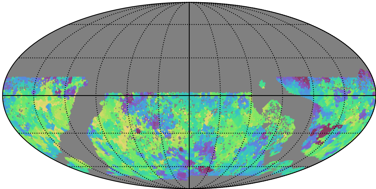
baseline_v3.0_10yrs WFD u band: Min saturation_mag
