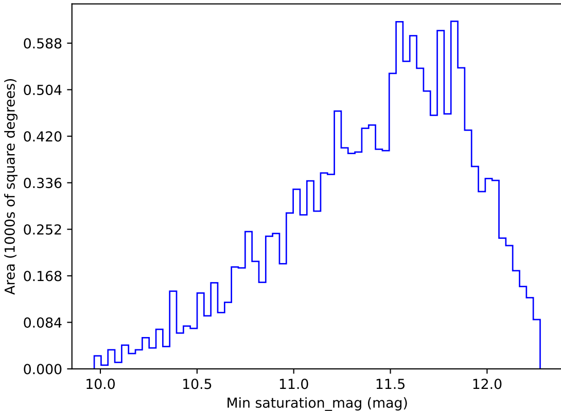
baseline_v3.0_10yrs WFD u band: Min saturation_mag
